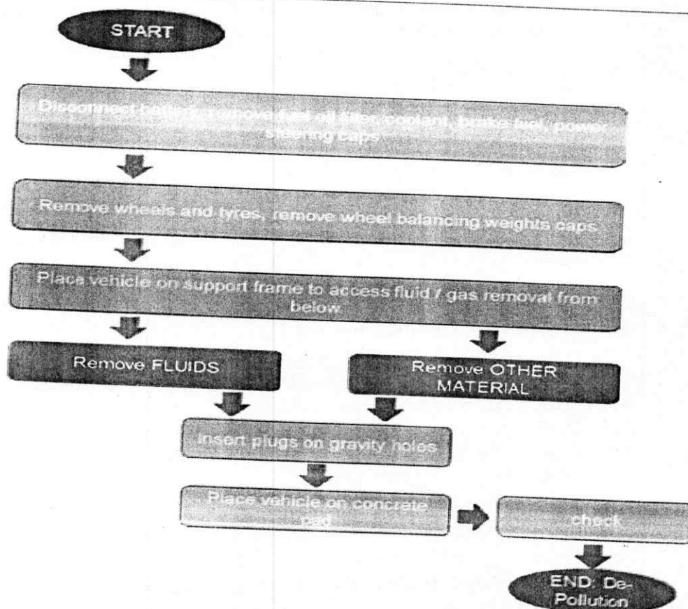
Figure 2: De-pollution process
